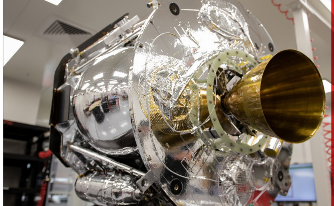
PHOTON INTERPLANETARY SPACECRAFT FOR NASA CAPSTONE LUNAR MISSION 2021
